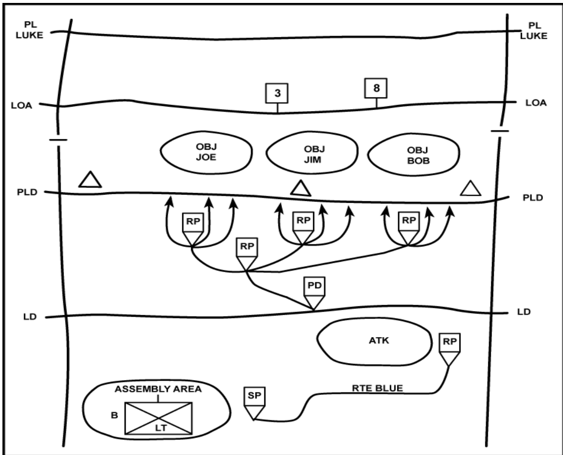
Figure 4-21. Linear assault.
