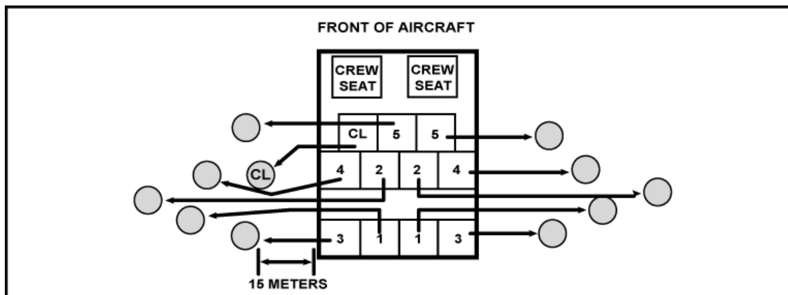
Figure D-1. UH-60 unloading diagram.
